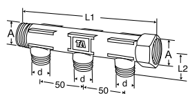
TA 56 043, 3-way distributor With swivelling nut
