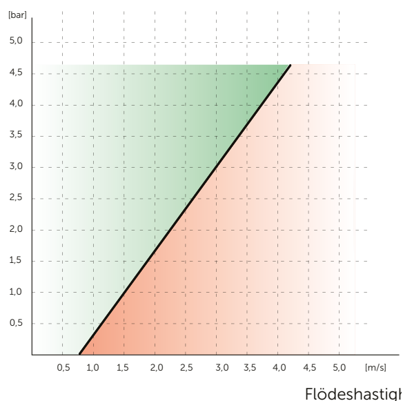
Systemtryck
