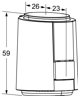
EMO T* – 230 VAC Including snap-on ring.
