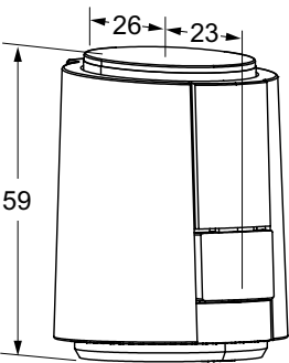
EMO T II – 24 VAC/VDC Including snap-on ring.
